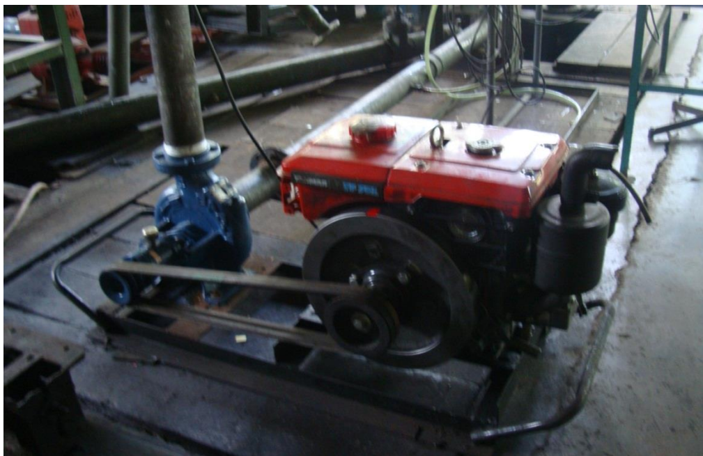
Figure 1. EAGLE EC80 Centrifugal pump coupled to YANMAR TF70L Diesel engine on the test set-up
