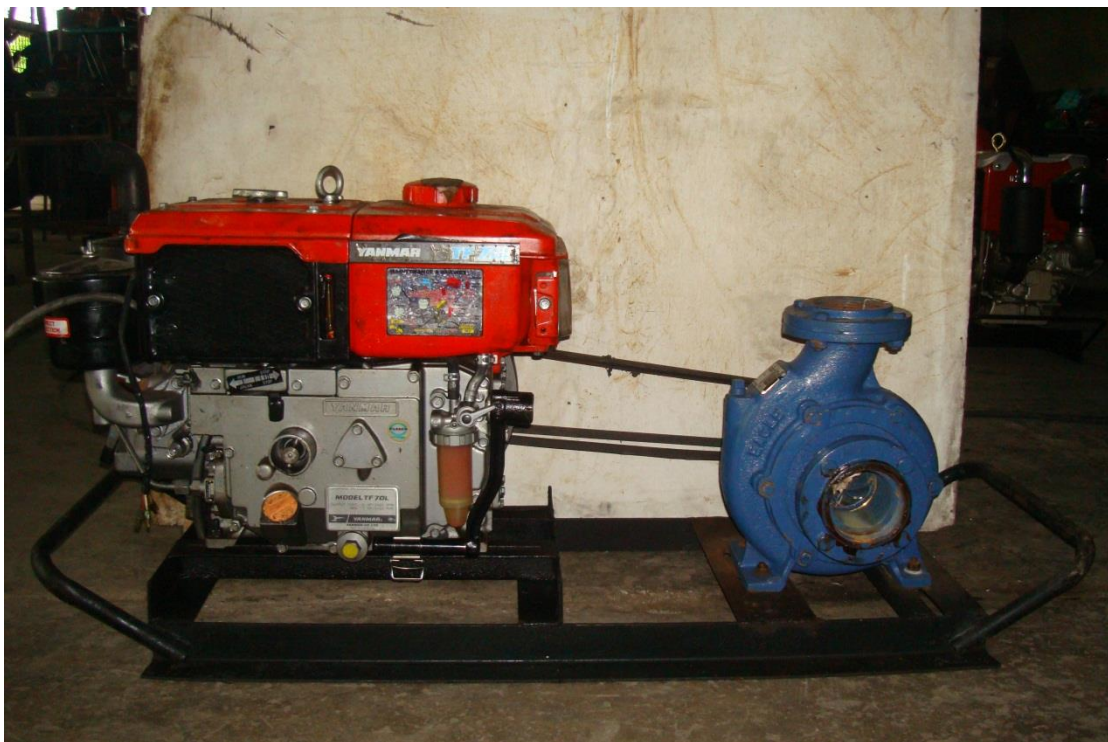
Figure 2. EAGLE EC80 Centrifugal Pump coupled to a YANMAR TF70L Diesel Engine
