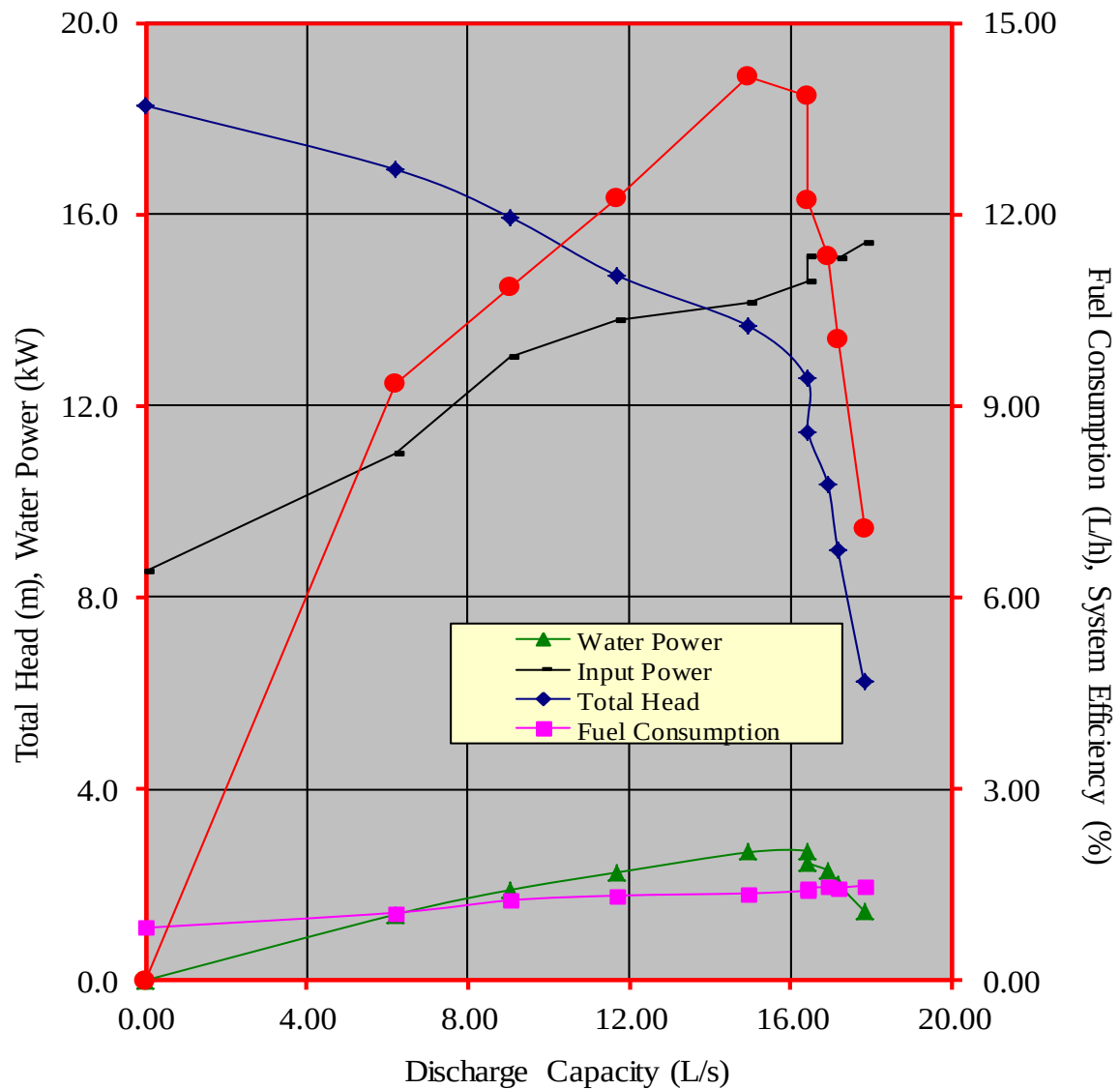
Figure 2. Performance characteristic curves of the EAGLE EC80 Centrifugal Pump coupled to a YANMAR TF70L Diesel Engine
